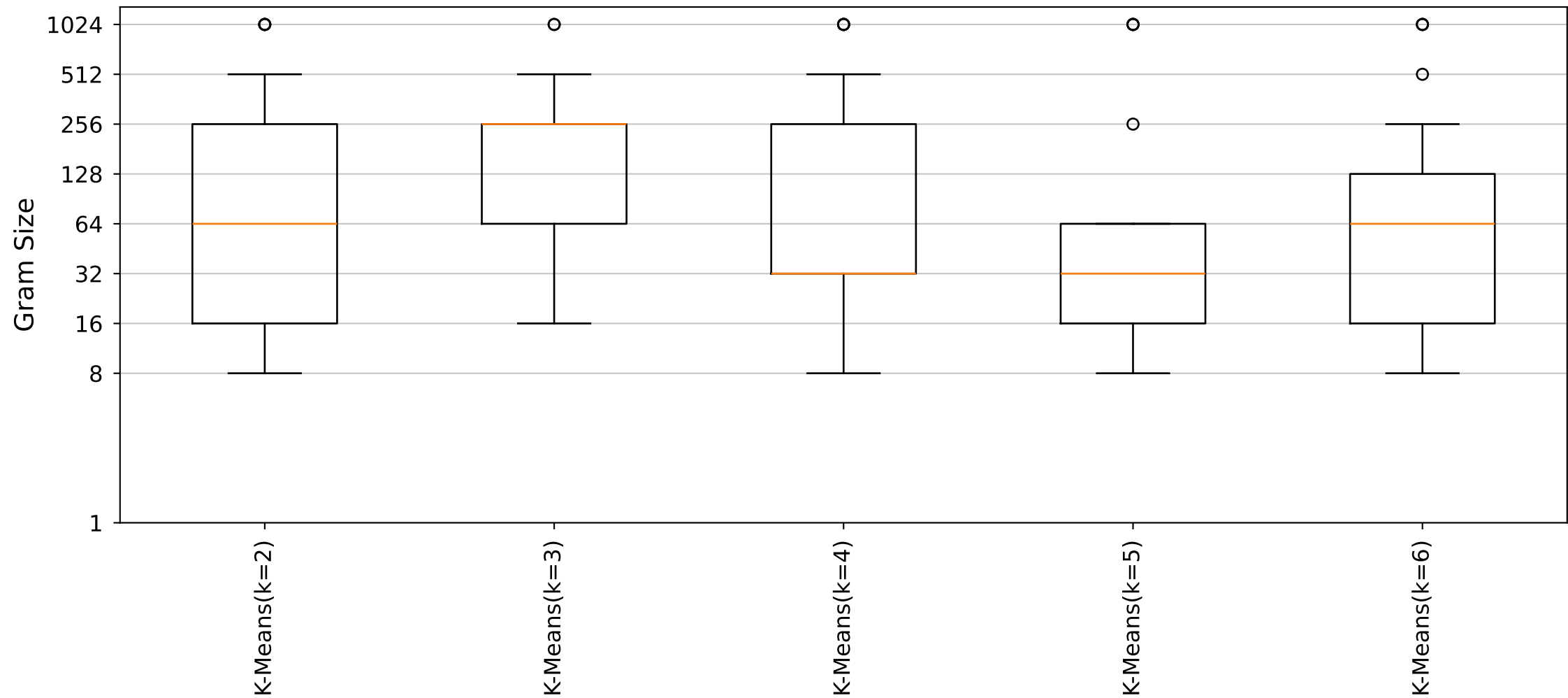
YARA Rules Gram Size Distribution (Cluster30_Size6 dataset)
